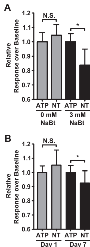
Fig. 4. Comparison of relative peak [\text{Ca}^{2+}]_{\text{cyt}} in differentiated and undifferentiated HT-29 cells stimulated with ATP or NT. A, normalized relative peak [\text{Ca}^{2+}]_{\text{cyt}} in cells treated with 0 or 3 mM NaBt. B, normalized relative peak [\text{Ca}^{2+}]_{\text{cyt}} in cells cultured for 7 days post-confluence. Data are mean \pm SEM ( n = 12 ) from four independent assays and are normalized to the ATP for each condition. Symbol (*) indicates significant difference; P < 0.05 using unpaired t -test.
